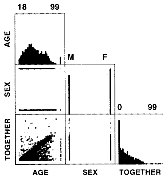
Figure 1 Scatter-Plot Matrix
